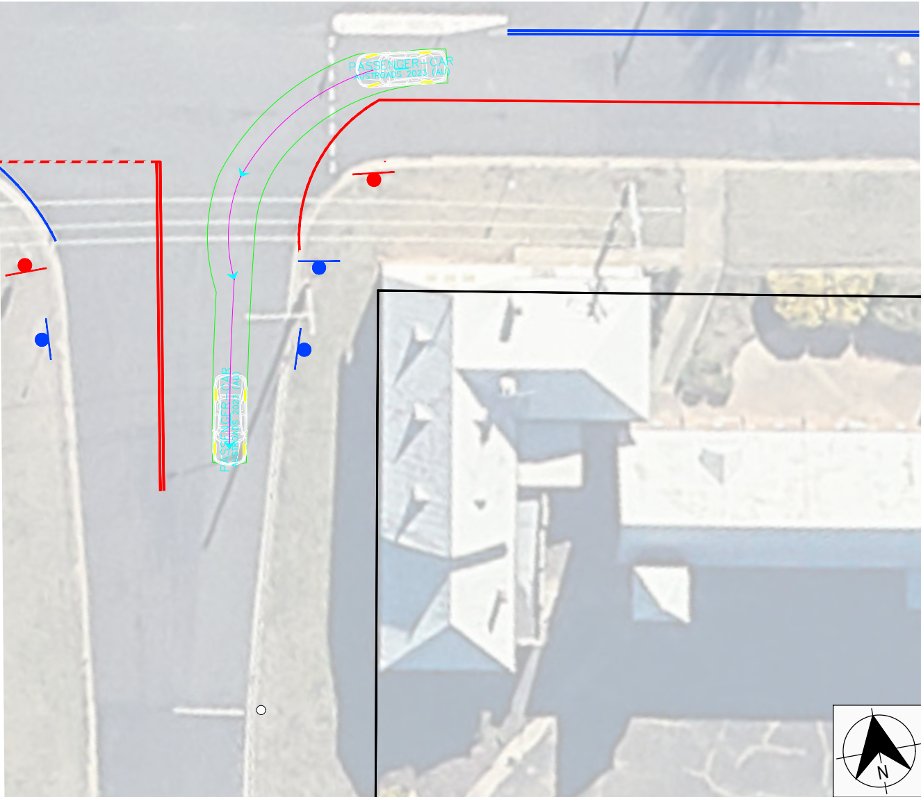
CAR TURNING PATH SCALE 1:100
