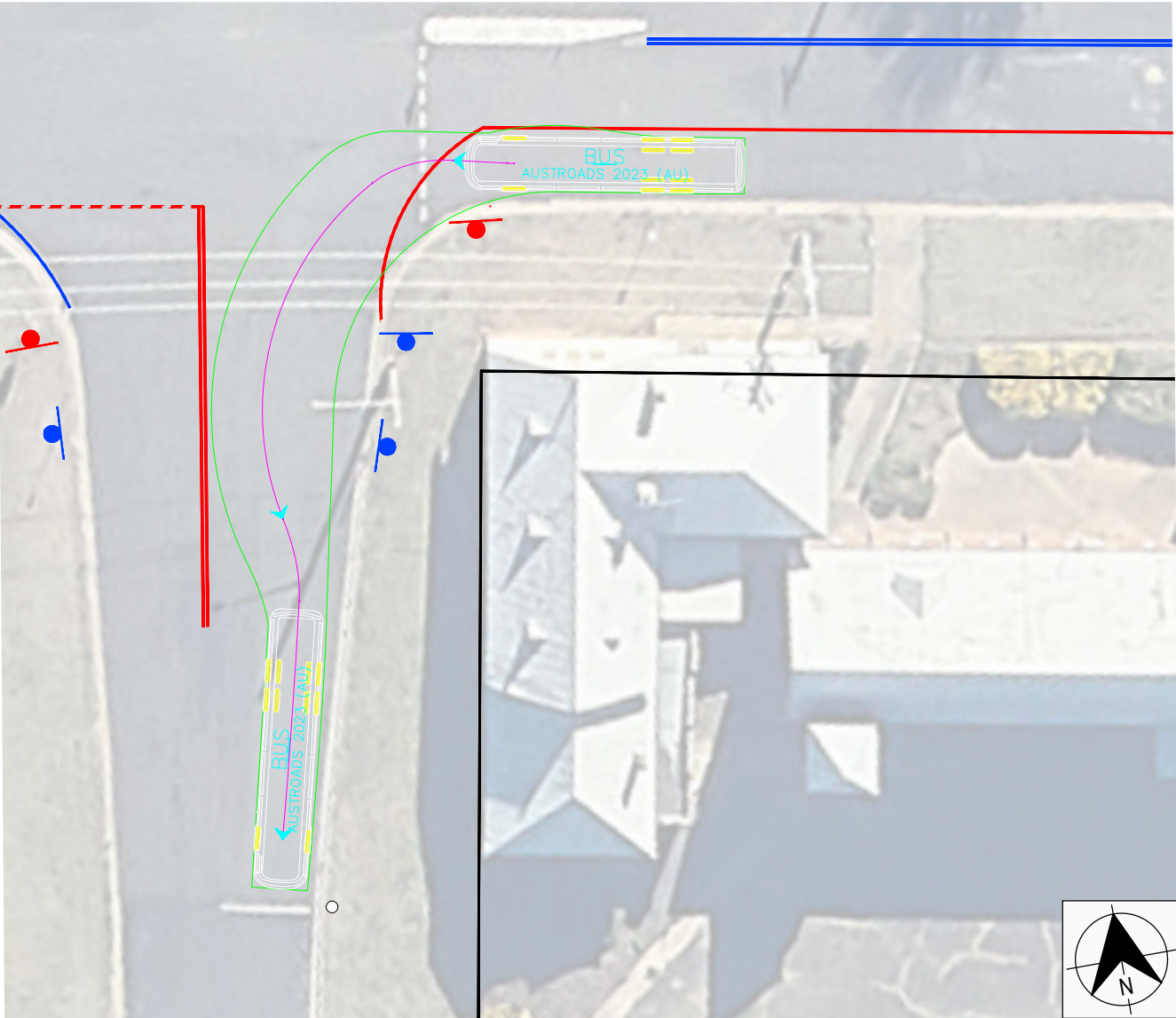
BUS TURNING PATH SCALE 1:100
